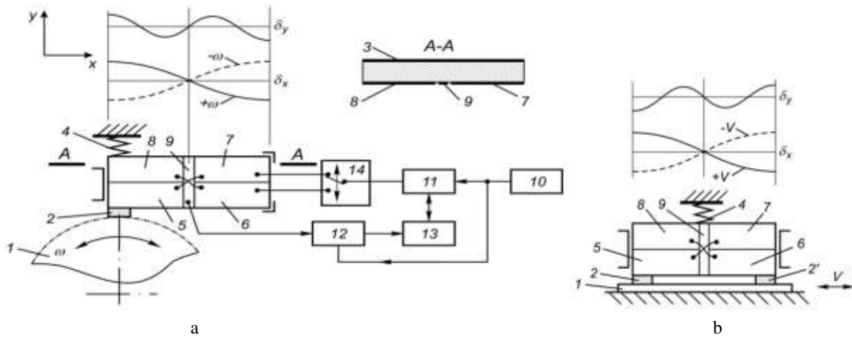
Fig. 1 Schemes of rotation (a) and translation (b) motion, which enables the diagnostics of tribological properties of piezoelectric motors' contact zone: 1 – rotor (1b – slipper), 2 – frictional contact element, 3 – plate-form piezoelectric transducer, polarised according to the plate thickness, 4 – spring, 5, 6, 7, 8 – symmetric electrodes sectioned by the transducer, 9 – central electrode for the measurement of electric charge, 10 – generator of harmonic signals, 11 – control unit, 12 – filter, 13 – detector/recorder
