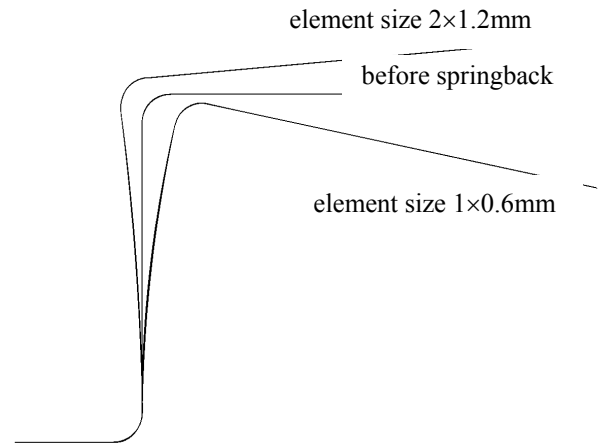
Fig. 15 Mesh size sensitivity
