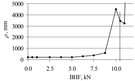
Fig. 6 Radius \rho versus BHF
