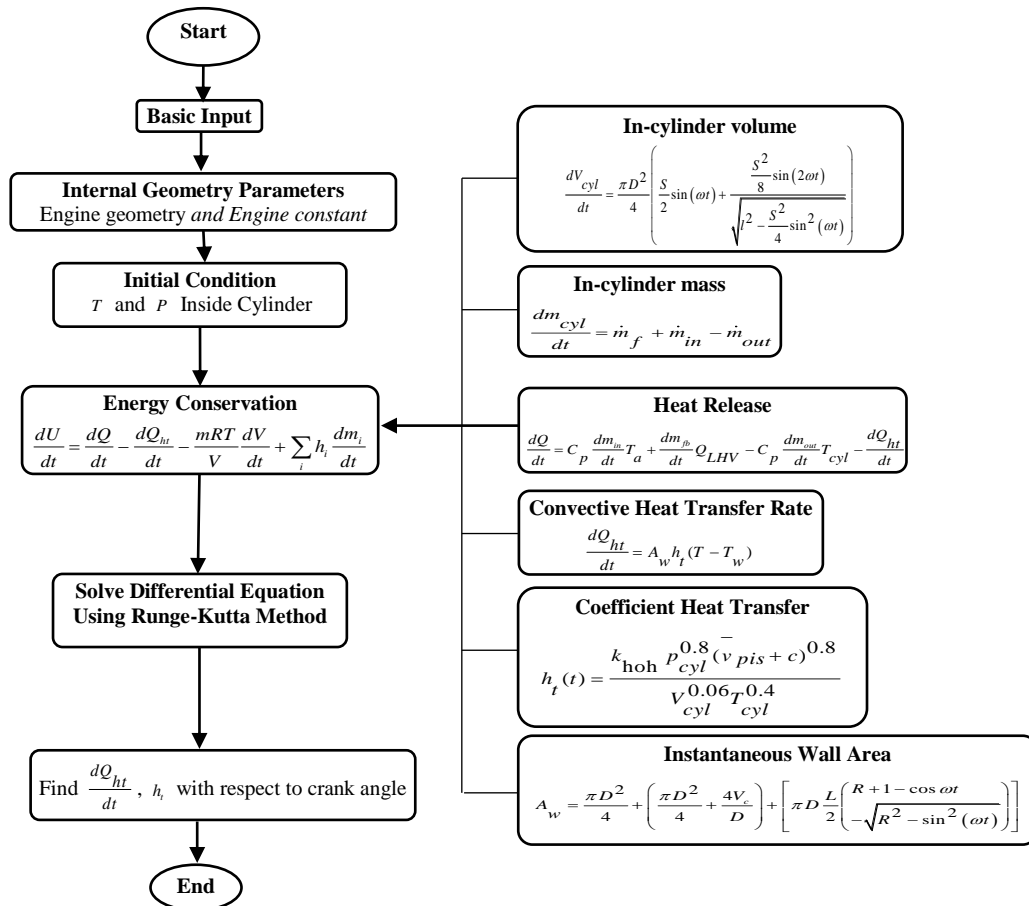
Fig. 2 Organization chart of a 6-cylinder turbocharged diesel engine modeling process
