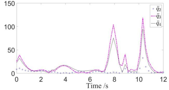
Fig. 15 Variation law of the angular acceleration \ddot{q}_i ( i=2,3,4 )
