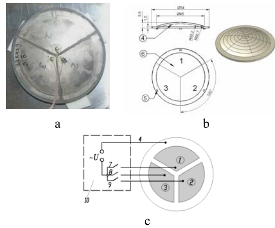
Fig. 3 2 DOFs positioning actuator No 3 (a), its drawing (b) and scheme of electric circuit (c)
