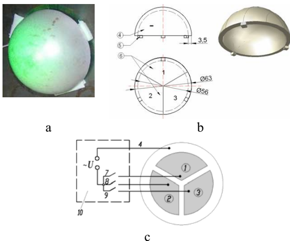
Fig. 1 2 DOFs positioning actuator No 1 (a), its drawing (b) and scheme of electric circuit (c)
