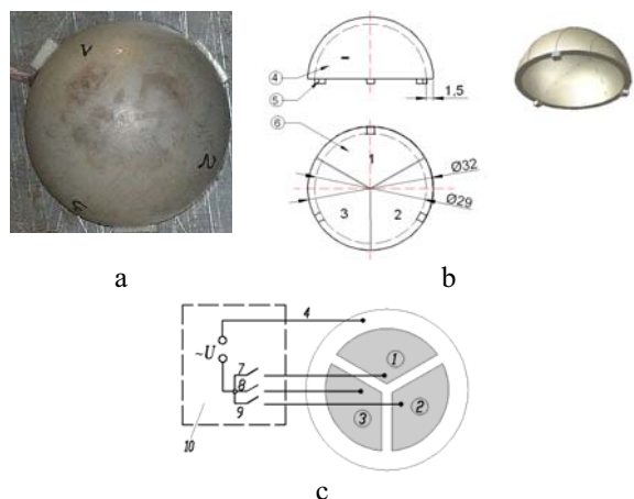
Fig. 2 2 DOFs positioning actuator No 2 (a), its drawing (b) and scheme of electric circuit (c)
