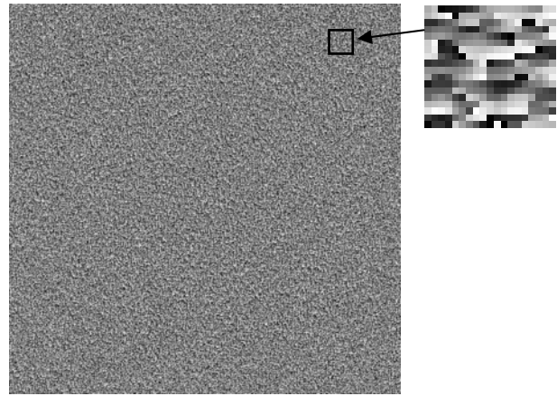
Fig. 2 Computer-generated hologram
