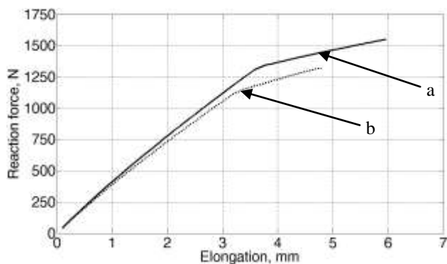
Fig. 3 The reaction force variation of the specimen: a - the specimen without implant, b - the specimen with the piezoelectric implant
