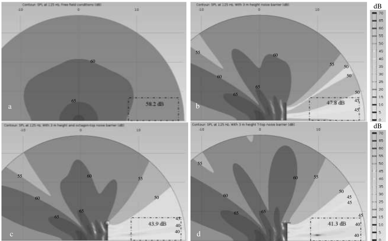
Fig. 6 Simulated acoustic field transformations at 125 Hz in a) free field conditions, b) with 3 m height noise barrier, c) with 3 m height noise barrier and octagon top d) with 3 m height noise barrier and T-shape top
