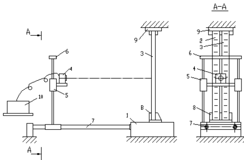
Fig. 1 Calibration equipment of levelling meters
