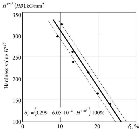
Fig. 10 The link between hardness value, when indenting conical indenter 2\theta=120^\circ , H^{120^\circ} and relative elongation \delta_i , in tension
