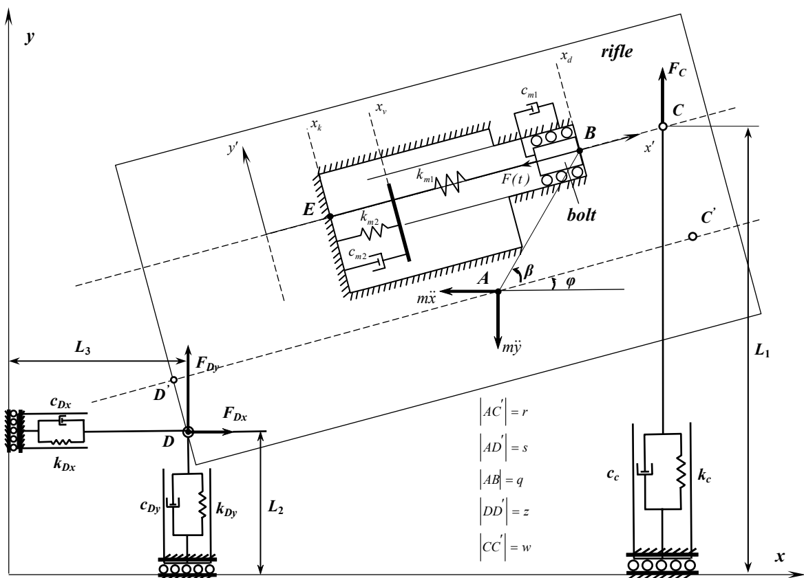
Fig. 1 Diagram of forces acting on the weapon
