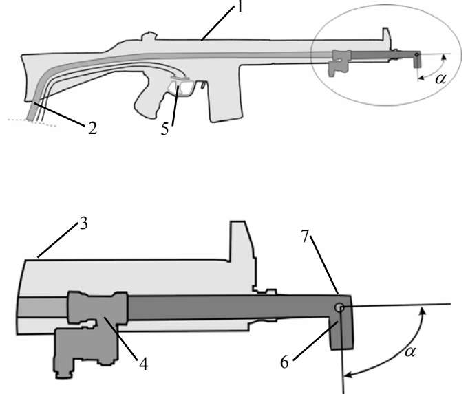
Fig. 3 Scheme of recoil imitation system of the rifle: 1 - rifle; 2 - feeding system of compressed air; 3 - barrel chamber; 4 - electromagnetic valve; 5 - trigger; 6 - discharge nozzle; 7 - position regulator of discharge nozzle
