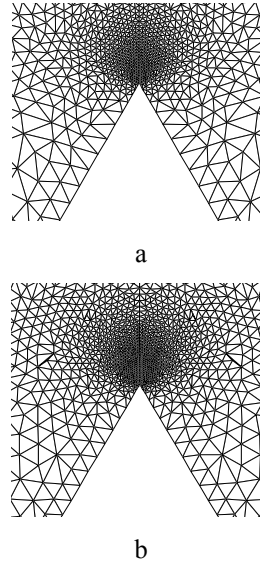
Fig. 5 Details of the adaptive FE meshes: a – 8th (3023 nodes, 5750 FE); b – 9th (3317 nodes, 6340 FE)
