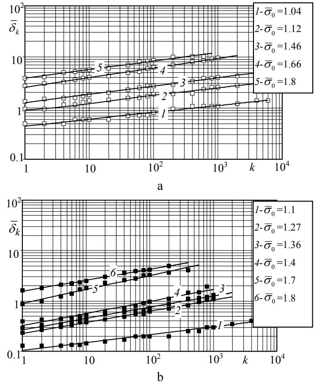
Fig. 7 Dependence of width of hysteresis loops on semicycle number k and load level \bar{\sigma}_0 , at low cycle pure bending: a – non hardened steel; b – hardened steel
