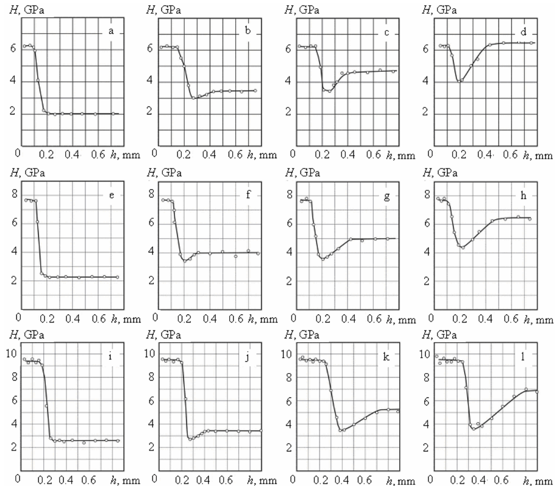
Fig. 2 Depth profiles of the average microhardness in surface layers of the steels: (a-d) grade 40; (e-h) grade 45; (i-l) grade U7 subjected to EMT after different preliminary HTs: quenching followed by tempering at (a, e, i) - 700; (b, f, j) - 500; (c, g, k) - 300; (d, h, l) - 150°C [7]
