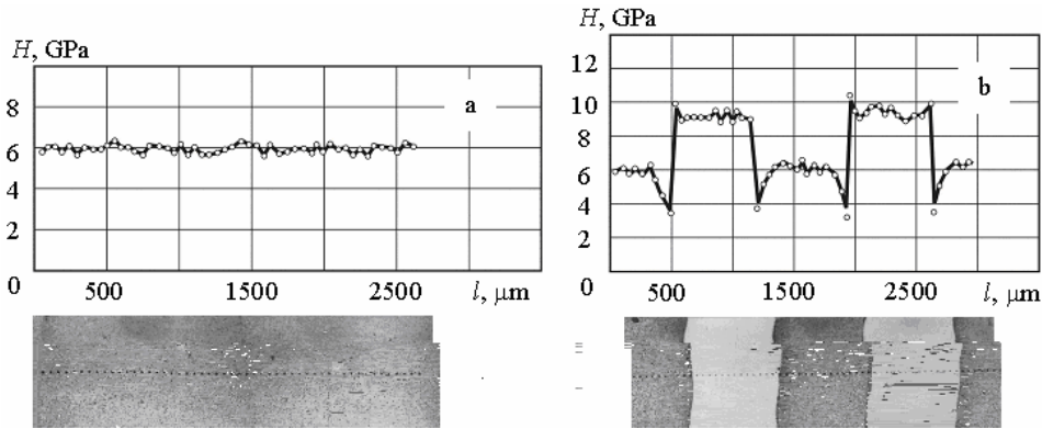
Fig. 4 Microhardness H distribution over the surface of the grade 45 steel along its axis l : (a) at the initial state; (b) after EMT at a gap of \sim 0.7 mm between white-layer tracks
