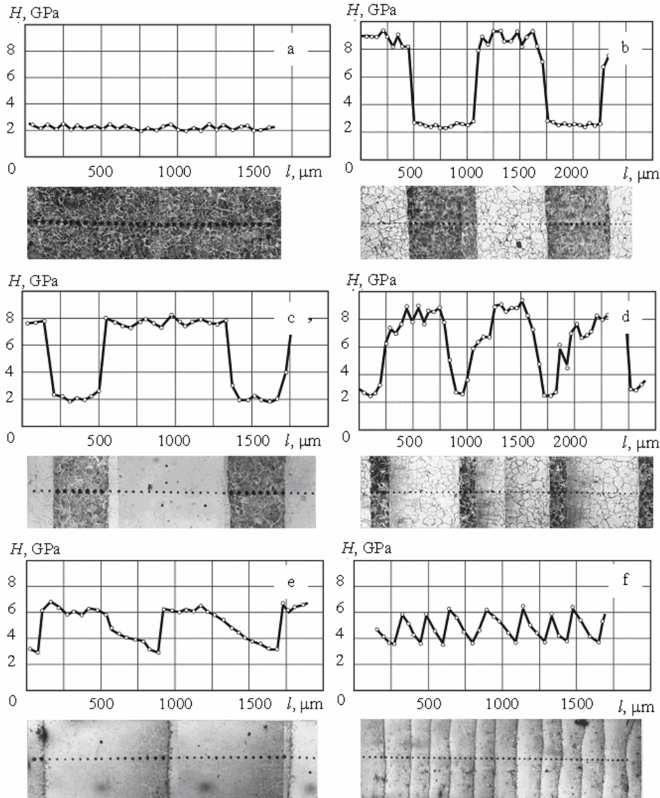
Fig. 3 Microhardness H distribution over the surface of the grade 45 steel along its axis l : (a) at the initial state and after EMT with various relative positions of white layer tracks; the gap between the tracks is (b) \sim 0.7 ; (c) \sim 0.3 (tempering zones are absent); (d) \sim 0.2 mm (tempering zones appear); (e) the tracks touch each other; (f) the tracks overlap each other
