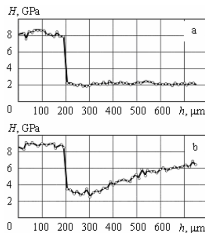
Fig. 1 Depth profiles of the average microhardness in the surface layers of the grade 45 steel samples subjected to EMT after (a) normalization and (b) quenching
