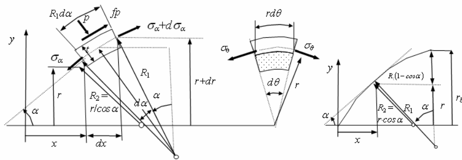
Fig. 5 Dimensions of a volume element of the shell of rotational symmetry and stresses acting on the volume element
