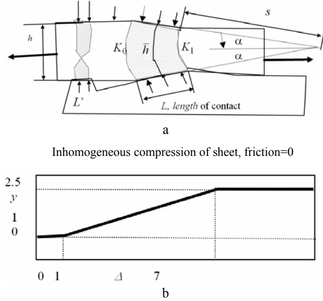
Fig. 2 Principles in a deformation process: a - geometry b - y vs \Delta schematically
