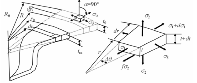
Fig. 3 Sheet flange deformation
