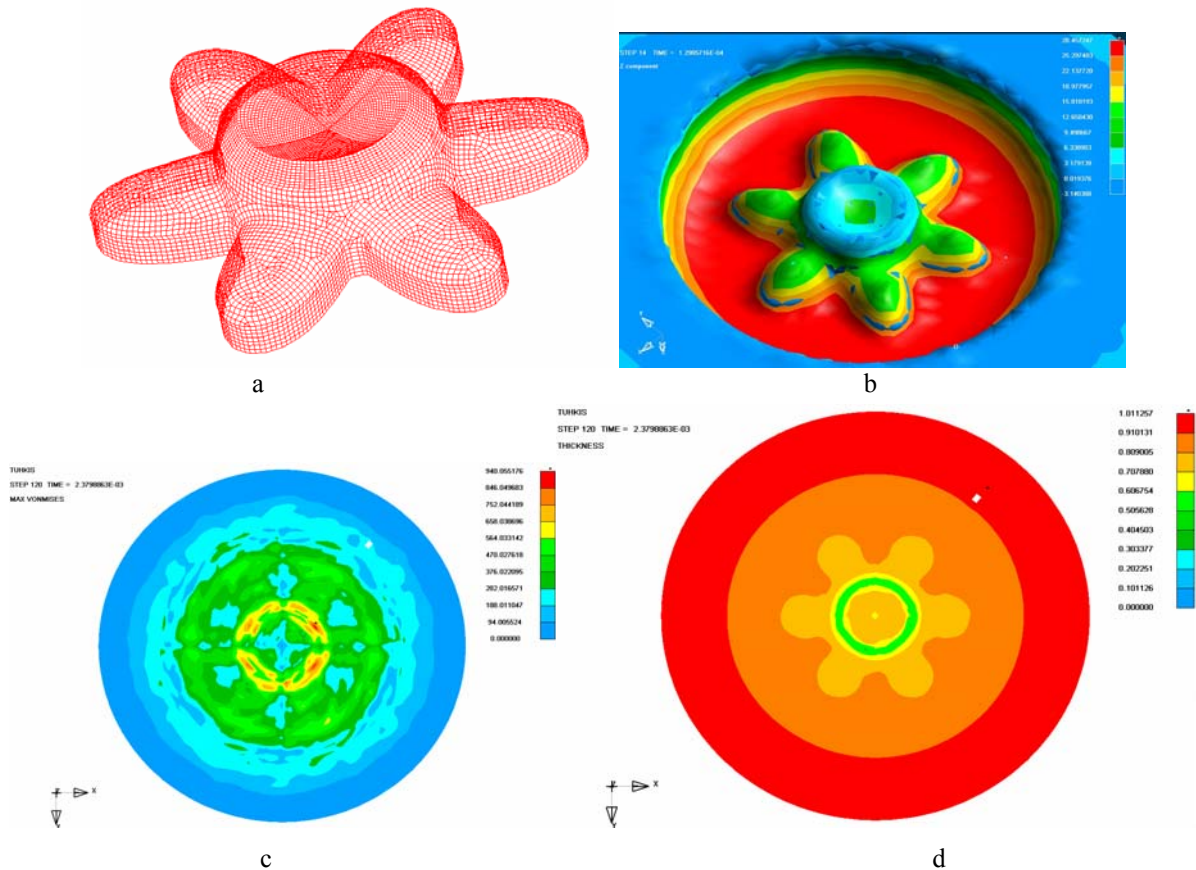
Fig. 6 Simulation results by LS-DYNA: a - the FEM mesh of the design-product; b - vertical z-depth contours; c - Von Mises stress contours at the final step (120). Max stress is 940MPa; d - thickness contours. The initial thickness is 1 mm. The mid cup bottom t/t_0 ratio is 0.7, the rim ratio is 0.5 and the outer cup model has ratio of 0.7-0.8. Rim ratio is 0.5 and the outer cup model has ratio of 0.7-0.8
