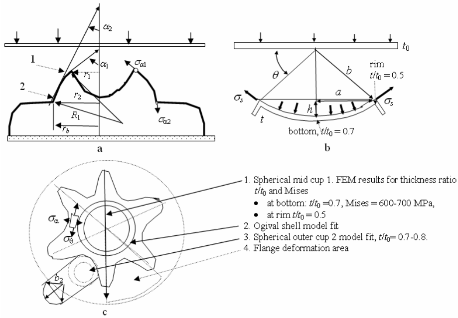
Fig. 4 Schematic models of the product (step 120): a - schematic cross section of the product; b - cup model; c - view from above
