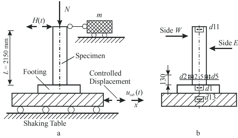
Fig. 2 Illustration of experiment: a - geometry of the specimen and forces, b - location of the displacement transducers
