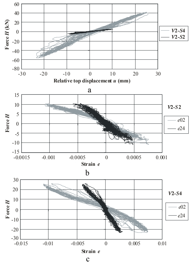
Fig. 3 Force-displacement curves on the specimen V2 at stages S2 and S4 : a - global behaviour H - u_G ; b, c - local behavior H - e_{ij}
