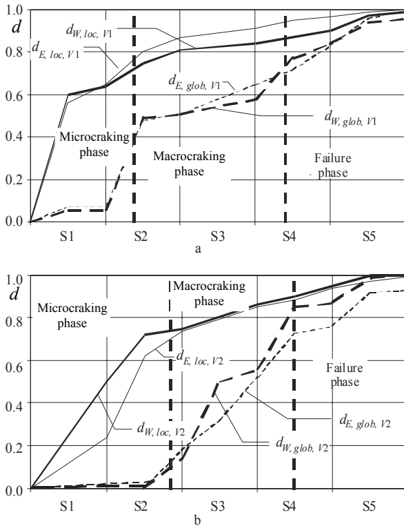
Fig. 6 Envelopes of damage indices for specimens V1 (a) and V2 (b)
