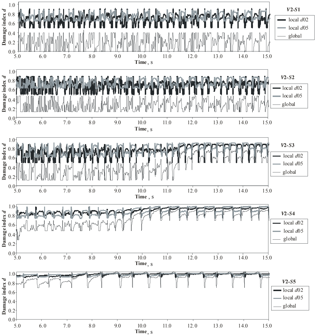
Fig. 5 Variation of the damage indices for specimen V2 at various loading stages
