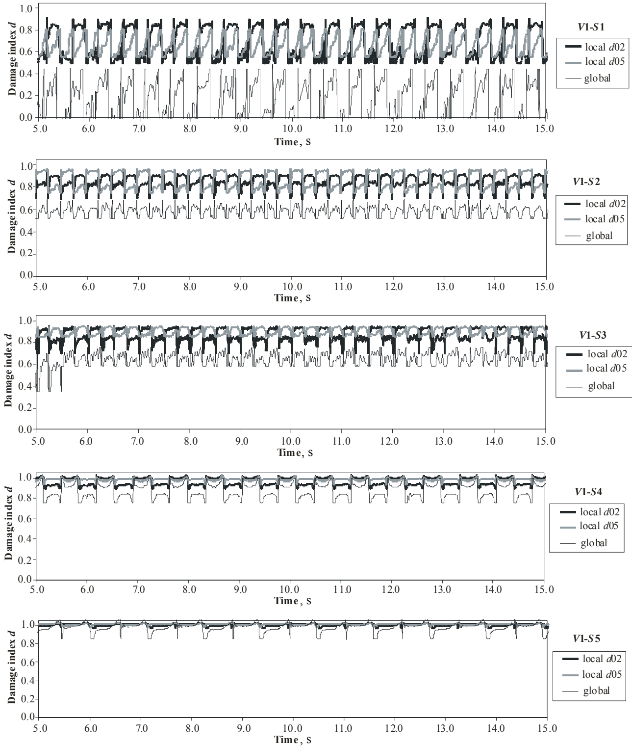
Fig. 4 Variation of the damage indices for specimen V1 at various loading stages
