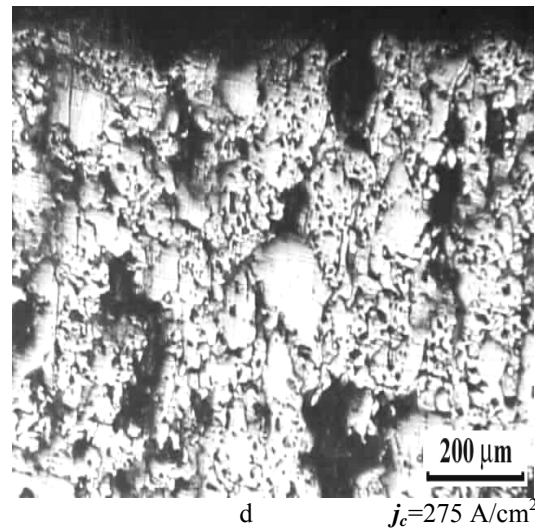
Fig. 2 Friction surface of Cu-10% vol graphite –70% vol. Gadfield steel composite (a-c) and commercially available MMC in the plane perpendicular to the direction of sliding (d) (black fields – graphite and/or pores)
