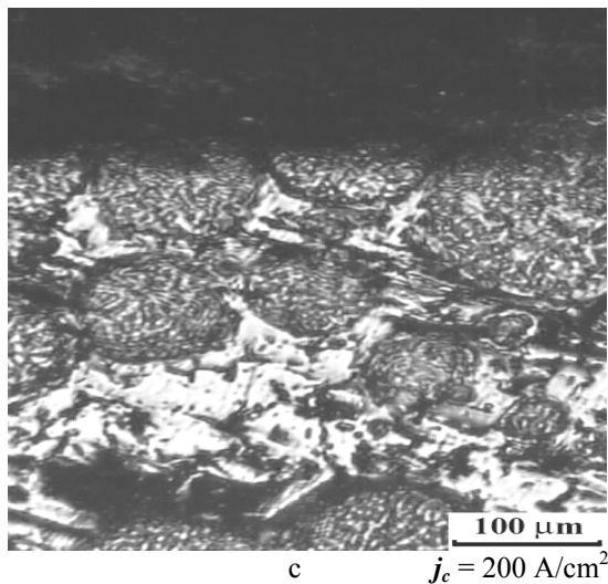
Fig. 2 Friction surface of Cu-10% vol graphite –70% vol. Gadfield steel composite (a-c) and commercially available MMC in the plane perpendicular to the direction of sliding (d) (black fields – graphite and/or pores)
