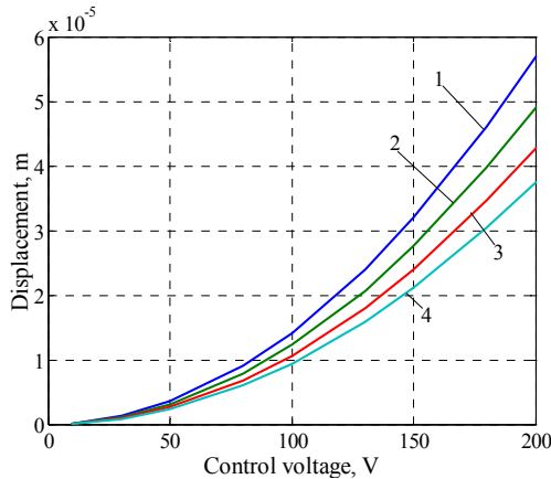
Fig. 4 Four turns Archimedes curve spring: 1- a gap between the plates -130 \mu\text{m} ; 2-a gap between the plates - 140 \mu\text{m} ; 3 - a gap between the plates - 150 \mu\text{m} ; 4- a gap between the plates- 160 \mu\text{m}
