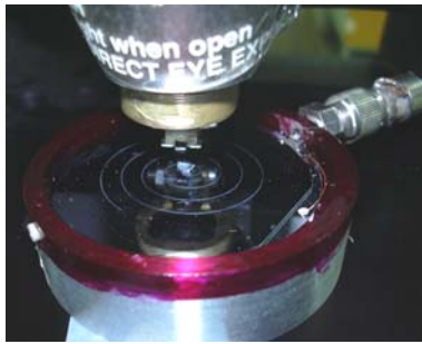
Fig. 9 Experimental setup for AFM investigations
