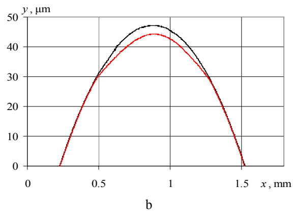
Fig. 8 Profilegrams of the middle of a rod : a - rod having modified surface AK; b - reference rod
