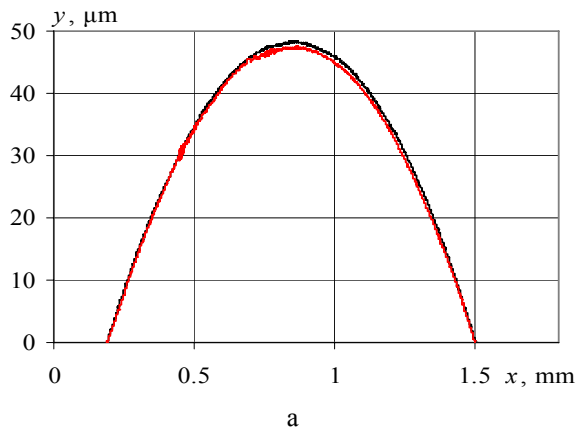
Fig. 7 Profilegrams of the front of a rod: a - rod having modified surface AK; b - reference rod
