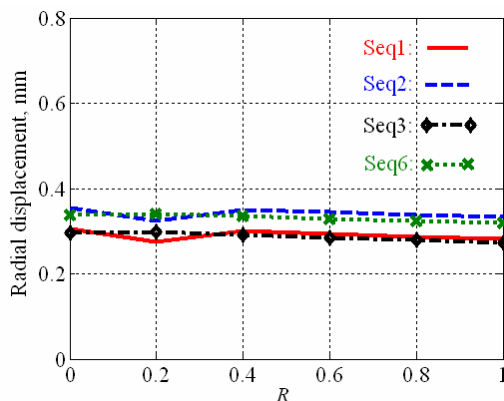
Fig. 9 Variations of the radial displacement through the thickness
