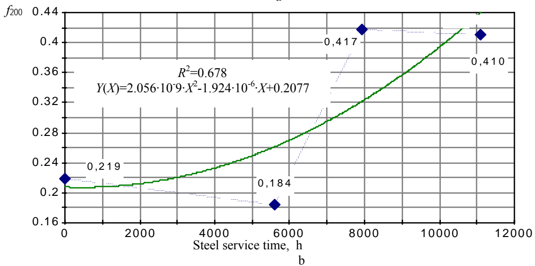
Fig. 4 The relationships of changing multifractal parameters depending steel service time: a - order ( \Delta ); b - uniformity ( f_{200} )
