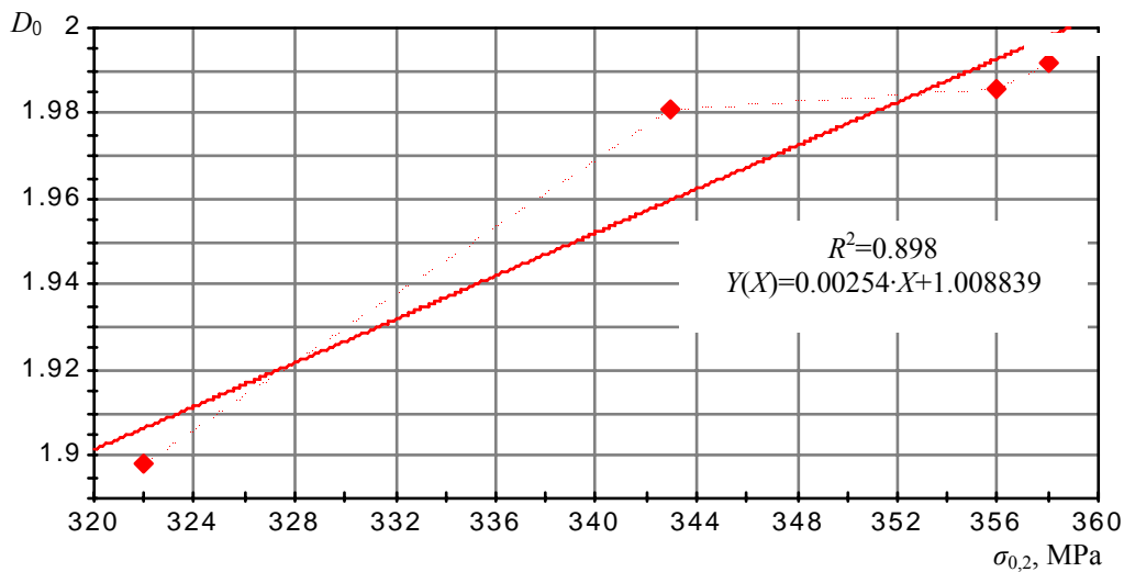
Fig. 5 Correlation of relative change of yield strength value with multifractal characteristic D_0 of steel containing 0.20% of carbon, 23% of chrome, 18% of nickel structure with various service time
