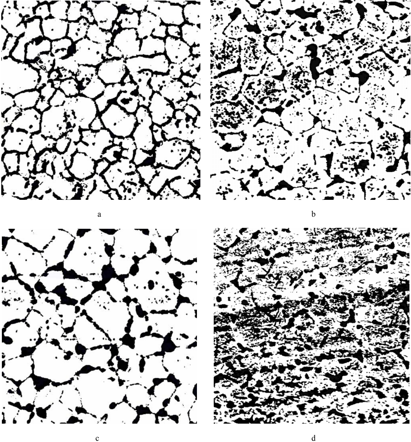
Fig. 3 Steel containing 0.20% of carbon, 23% of chrome, 18% of nickel structure: a - 0 h; b - 5605 h; c - 7929 h; d - 11082 h
