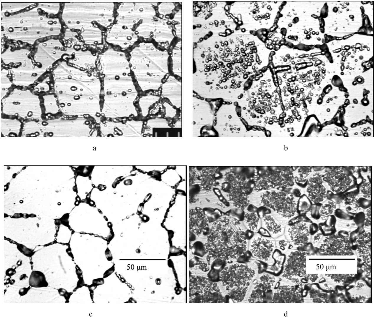
Fig. 2 Steel sample structure containing 0.20% of carbon, 23% of chrome, 18% of nickel, \times 1700 : \tau = 0 h; \tau = 5605 h; \tau = 7929 h; \tau = 11082 h
