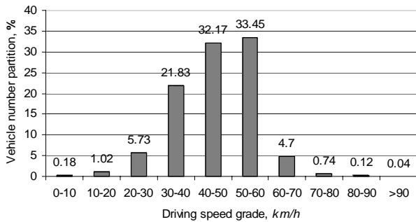
Fig. 1 The partition of street traffic flow based on the driving speed (K. Donelaičio str.)
