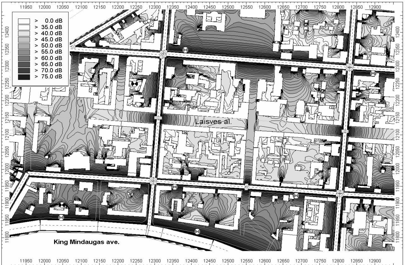
Fig. 3 The fragment of the street traffic noise map (predictive mapping, speed limit 60km/h)
