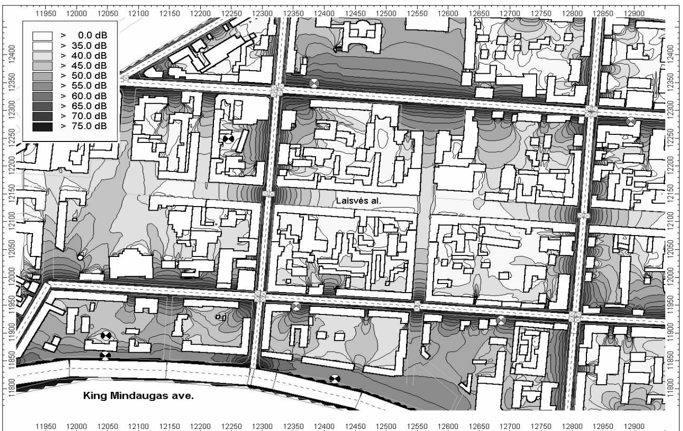
Fig. 4 The fragment of the street traffic noise map (predictive mapping, redistributed traffic flows)
