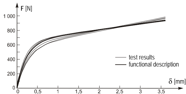
Fig. 6 Load-slip fastener characteristics for chipboard sheathing
