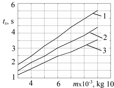
Fig. 17 Dependence of the time the part stops moving both on the bushing's mass m and friction coefficient \mu , as v=0.01 m/s, R_e=0.01 m, \omega=45 s -1 , c=15 N/m, h_x=h_y=0.2 Ns/m, c_x=c_y=10 N/m, \omega=45 s -1 : 1 - \mu=0.2 , 2 - \mu=0.25 , 3 - \mu=0.3
