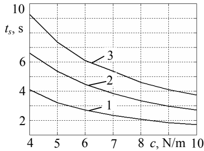
Fig. 15 Dependence of time as part stops on peg's pressing spring rigidity c and excitation amplitude R_e , as m=0.005 kg, v=0.005 m/s, h_x=h_y=0.2 Ns/m, c_x=c_y=10 N/m, \mu=0.3 , \omega=50 s -1 : 1 - R_e=0.005 m, 2 - R_e=0.0075 m, 3 - R_e=0.01 m
