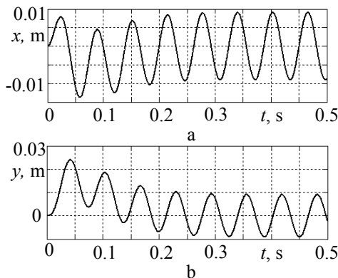
Fig. 2 Characteristic vibrations of the part, as m=0.01 kg, F=2 N, h_x=h_y=0.2 Ns/m, c_x=c_y=10 N/m, \mu=0.1 , R_e=0.01 m, \omega=200 s ^{-1} : a - along the x axis direction, b - along the y axis direction
