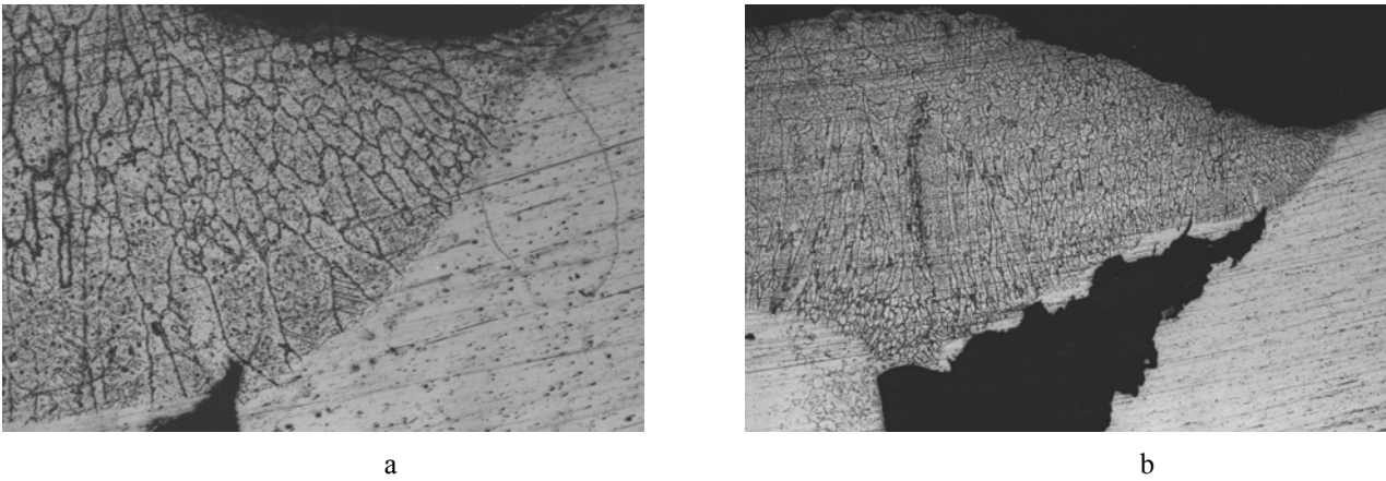
Fig. 5 Initial (a, x100) and final (b, x20) stages of the destruction of a welded seam received at welding grade 08X25T steel by austenitic electrodes OZL-6
