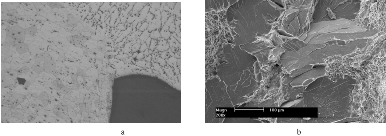
Fig. 6 Structure of a fusion zone (a, x200, left – basic metal, right – welded joints) and a fracturegram (b) of a welded seam received at welding grade 08X25T steel by austenitic-ferritic electrodes UTP-65D
