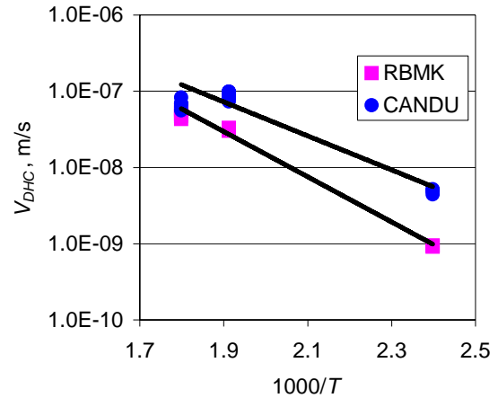
Fig. 2 DHC axial velocity data as a function of 1000/T
