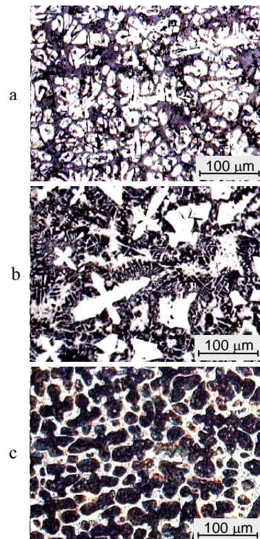
Fig. 1 Microstructure of lathe tool cutting unit subjected to overlay welding: a - welding under AMS1 flux with WC-8%Co powder spread over the tool surface; b - welding under AMS1 flux mixed with 33 % cast iron grinding waste powder and WC-8%Co powder spread over the tool surface; c - welding under the flux mixed with 4.5 % B 4 C and 4.5 % graphite powder and P6M5 steel chips spread over the tool surface
