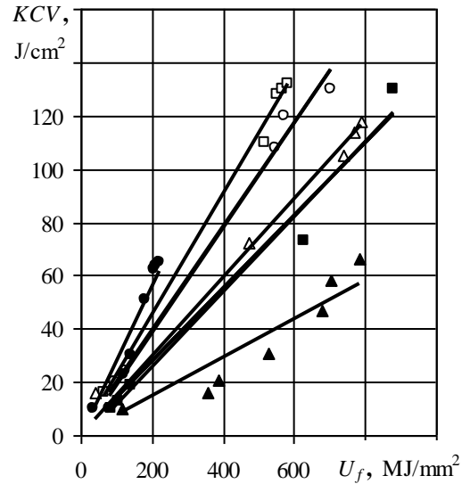
Fig. 4 Relationship between critical indentation energy U_f and impact strength, KCV : ● – 17G1S-U, □ – 06G2NAB, ○ – 10G2FB-U, Δ – 10HGNMAYu, ■ – 10G2FB, ▲ – 17GS
