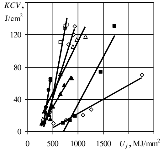
Fig. 3 Relationship between critical indentation energy U_f and impact strength, KCV : □ – 06G2NAB, ■ – 10G2FB, ○ – 10G2FB-U, Δ – 10HGNMAYu, ◇ – Vst3kp, ▲ – 17GS, ● – 17G1S-U
