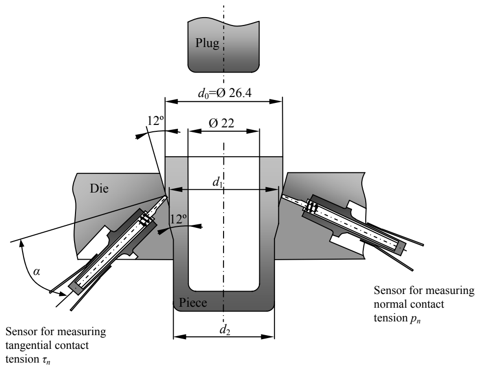
Fig. 2 Process of deep drawing with the system for measurement of contact tensions p_n and \tau_n
