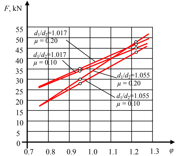
Fig. 5 Theoretical correlation between deep drawings force F , kN and deformation degree \varphi
