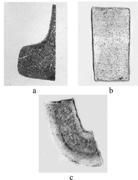
Fig. 4 Investigation of sulphur segregation in the separated railway elements: a – rail; b – sleeper; c – yoke of rail attaching
