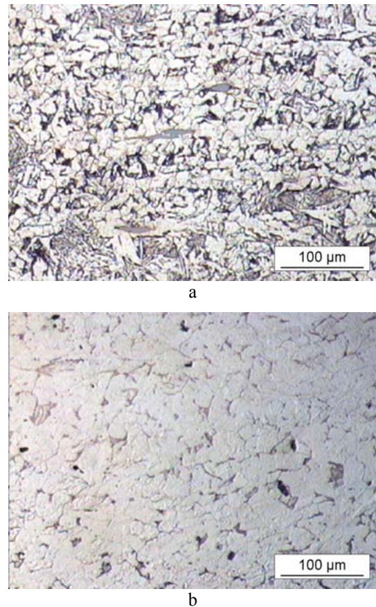
Fig. 3 Microstructure of rail attaching element: a – central part of specimen; b – decarbonized surface part of specimen
