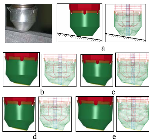
Fig. 13 Deformation of the detonator cap – views of the interaction with nondeformable surface at hitting angle \alpha = 80^\circ (on the left – experimental view, on the right – modelling results): a – initial position t = 0 , b – v = 35 m/s, c – v = 45 m/s, d – v = 52 m/s, e – v = 57 m/s
