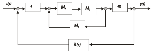
Fig. 5 Example of main circuit with power regulator
