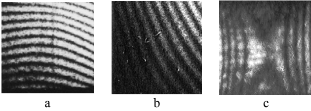
Fig. 16 Holograms of thermally deformed holographic plate fixed using universal (a), multiple (b) and angular fine adjustment (c) holders
