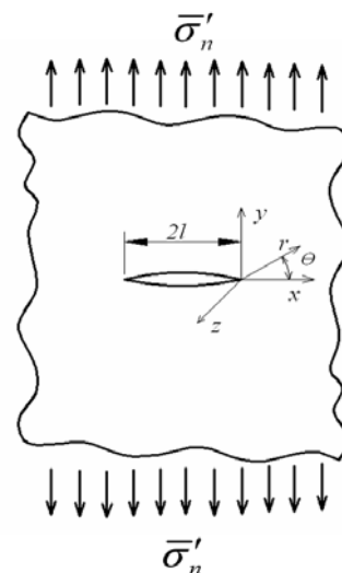
Fig. 1 The scheme of loading of infinite plate with a crack
