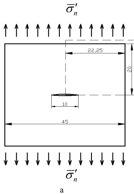
Fig. 2 Two-dimensional (2D) model with crack: a - model of plate with a crack for the FEM; b - the FEM mesh on the whole plate and in the zone of the stress concentration (measures indicated in mm)
