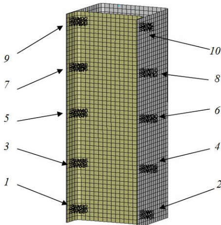
Fig. 11 Location and numeration of the spot-welding
