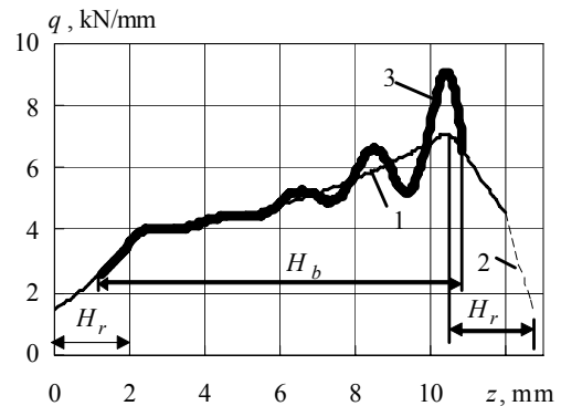
Fig. 6 Load distribution in the thread of tight stud at bending of the threaded joint M16: 1 - q_{st}(z) , 2 - q_{st}(z) on plastically deformed part of runout, 3 - q_{st}(z) = q_{st}(z) + q_{sb}(z)
