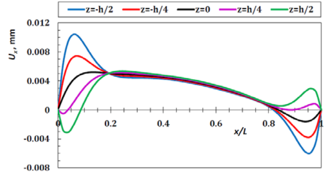
Fig. 2 Axial displacement distribution in different layers
