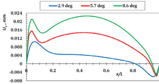
Fig. 6 Axial displacement distribution along inner surface with different tapering angles
