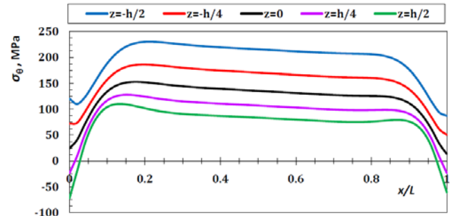
Fig. 4 Circumferential stress distribution in different layers
