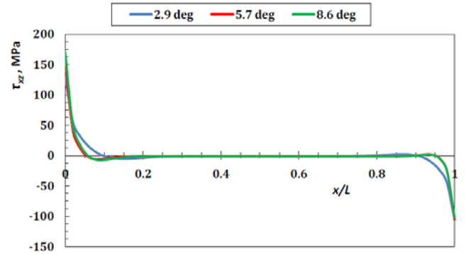
Fig. 9 Shear stress distribution along inner surface with different tapering angles
