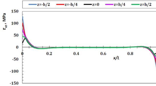
Fig. 5 Shear stress distribution in different layers
