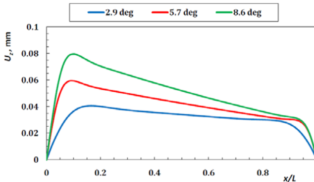
Fig. 7 Radial displacement distribution along inner surface with different tapering angles
