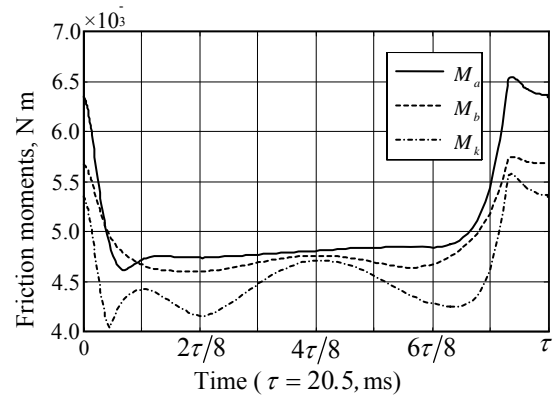
Fig. 10 Friction moments of the bearings
