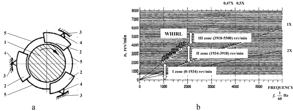
Fig. 4 Rotary system: a - adaptive hydrodynamic bearing with the segments connected with elastic strips: 1 - rotor, 2 - segments, 3 - body, 4 - adaptive tilting pad, 5 - elastic strips connecting segments; b - graph of resonant frequencies of rotary system, when clearance between rotor and bearing 50 \mu\text{m}
