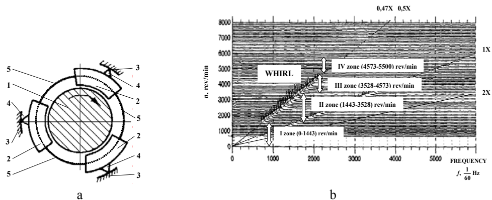
Fig. 5 Rotary system: a - adaptive hydrodynamic bearing with elastic ring that is moved easily and is connecting segments: 1 - rotor, 2 - segments, 3 - body, 4 - adaptive tilting pad, 5 - elastic ring; b - graph of resonant frequencies of rotary system, when clearance between rotor and bearing 50 \mu\text{m}
