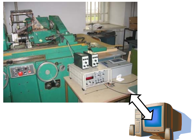
Fig. 2 Stand of experimental researches
