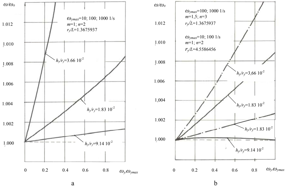
Fig. 3 Frequency response of angular velocity of the rotation of elastic ring: a - in the case of long elastic ring; b - in a case of the hydrodynamic suspension of short and long elastic elements
