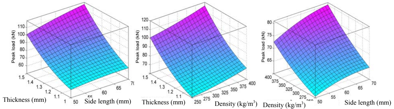
Fig. 5 Response surface of peak force for the foam filled spot welded column
