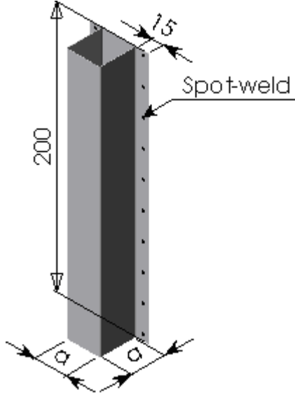
Fig. 1 Schematic drawings of the spot-welded column used in the current study
