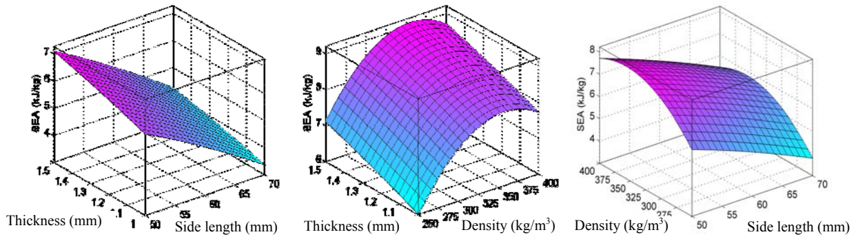
Fig.4 Response surface of SEA for the foam filled spot welded column
