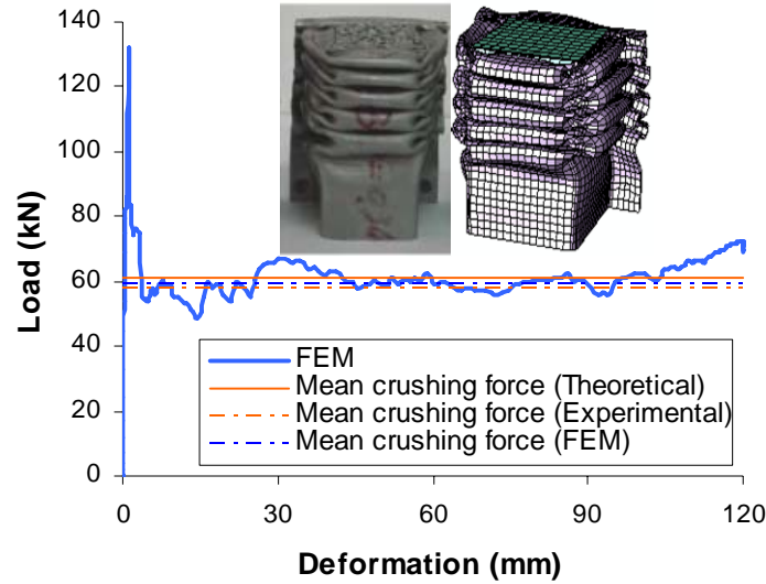
Fig. 3 Comparison of the experimental [5] and numerical result
