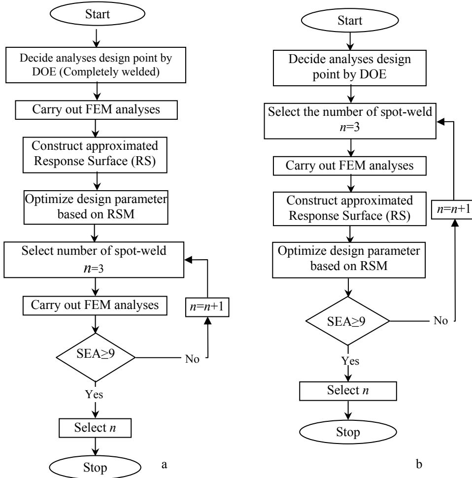
Fig. 2 Flowcharts of the two optimization processes: a - first algorithm, b - second algorithm
