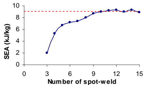
Fig. 7 Variation of the SEA vs. number of spot-welds
