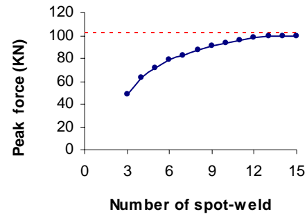
Fig. 6 Variation of the peak crushing force vs. number of spot-welds
