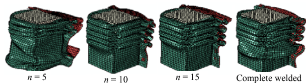
Fig. 8 Deformation of foam-filled spot-welded columns with various numbers of spot-welds
