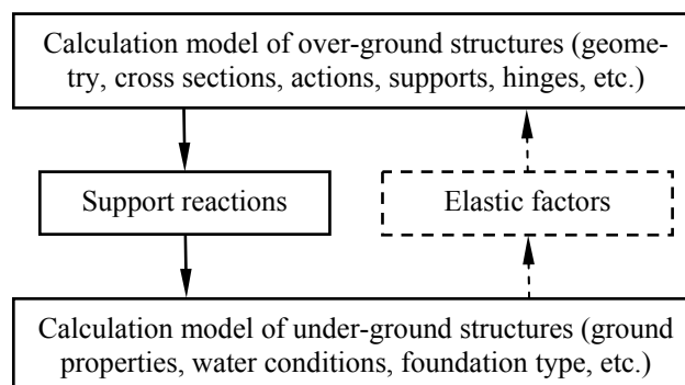
Fig. 1 Conventional model of the single-stage calculation in a simple structural design
