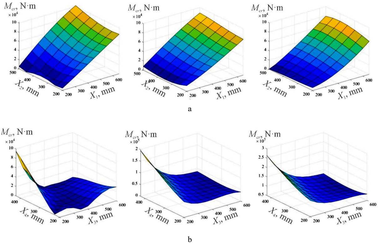
Fig. 5 Regression model of the carbody rotation moment relative to the instantaneous center of rotation: M_{cr} – carbody rotation moment relative to the instantaneous center of rotation: a – minimum, average, and maximum values of the coordinates of the lower attachment points of the carbody suspension levers; b – minimum, average, and maximum values of the coordinates of the upper attachment points of the carbody suspension levers
