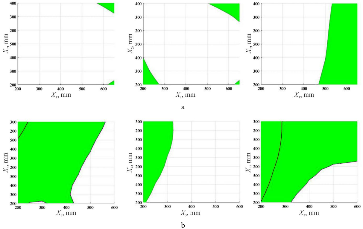
Fig. 4 Operability zones of the carbody tilting mechanism with respect to stability coefficient limits: a – minimum, average, and maximum values of the coordinates of the lower attachment points of the carbody suspension levers; b – minimum, average, and maximum values of the coordinates of the upper attachment points of the carbody suspension levers
