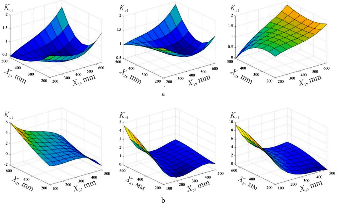
Fig. 3 Regression model of the stability coefficient: K_{c1} derailment stability coefficient; X_1 & X_2 – coordinates of the lower attachment points of the carbody suspension levers; X_3 & X_4 coordinates of the upper attachment points. a – minimum, average, and maximum values of the coordinates of the lower attachment points of the carbody suspension levers; b – minimum, average, and maximum values of the coordinates of the upper attachment points of the carbody suspension levers
