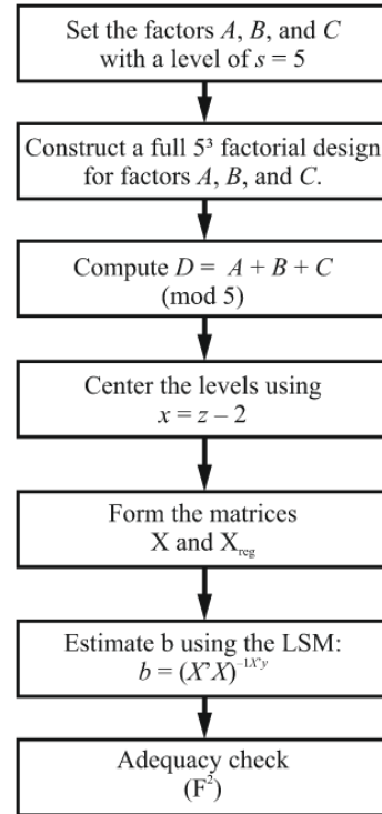
Fig. 1 Block diagram of the regression model calculation algorithm: A , B , C – independent factors; s – level of coordinate space; 5^3 – factorial design; D – factor determined by the experimental conditions; x – centered levels; z – initial levels; X – experimental matrix; X_{reg} – matrix of cubic regressors; b – regression coefficients; F^2 – model adequacy check
