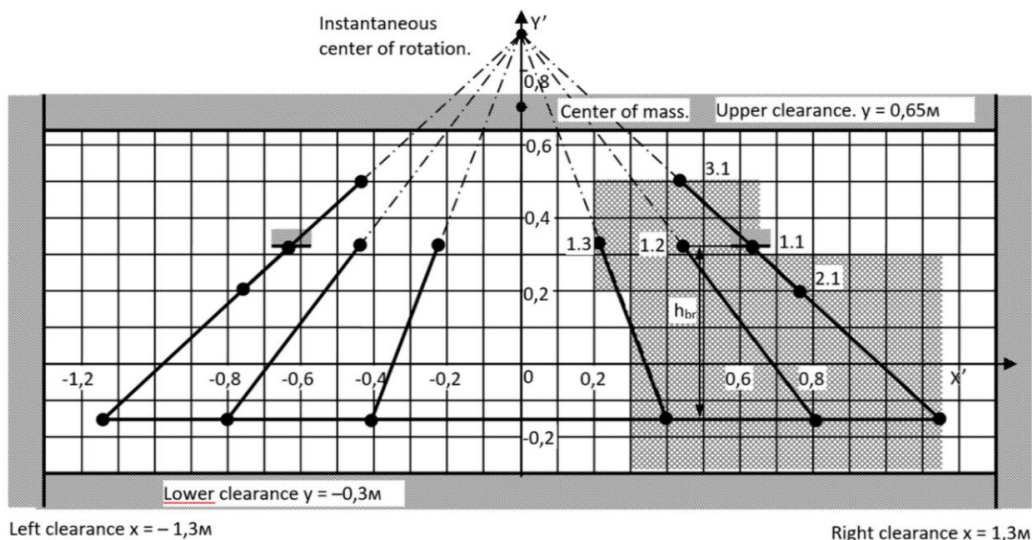
Fig. 2 Variation of the car body tilting mechanism configuration
