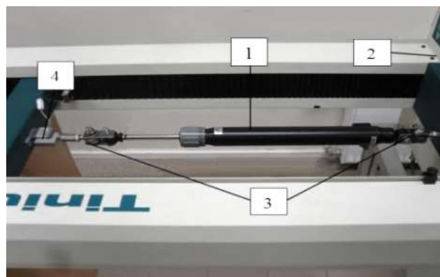
Fig. 3 Test rig for resistance force characteristics analysis of hydraulic cylinders: 1 – hydraulic cylinder; 2 – testing machine Tinius Olsen H25KT; 3 – spherical bearings; 4 – force sensor HTE-1000N
